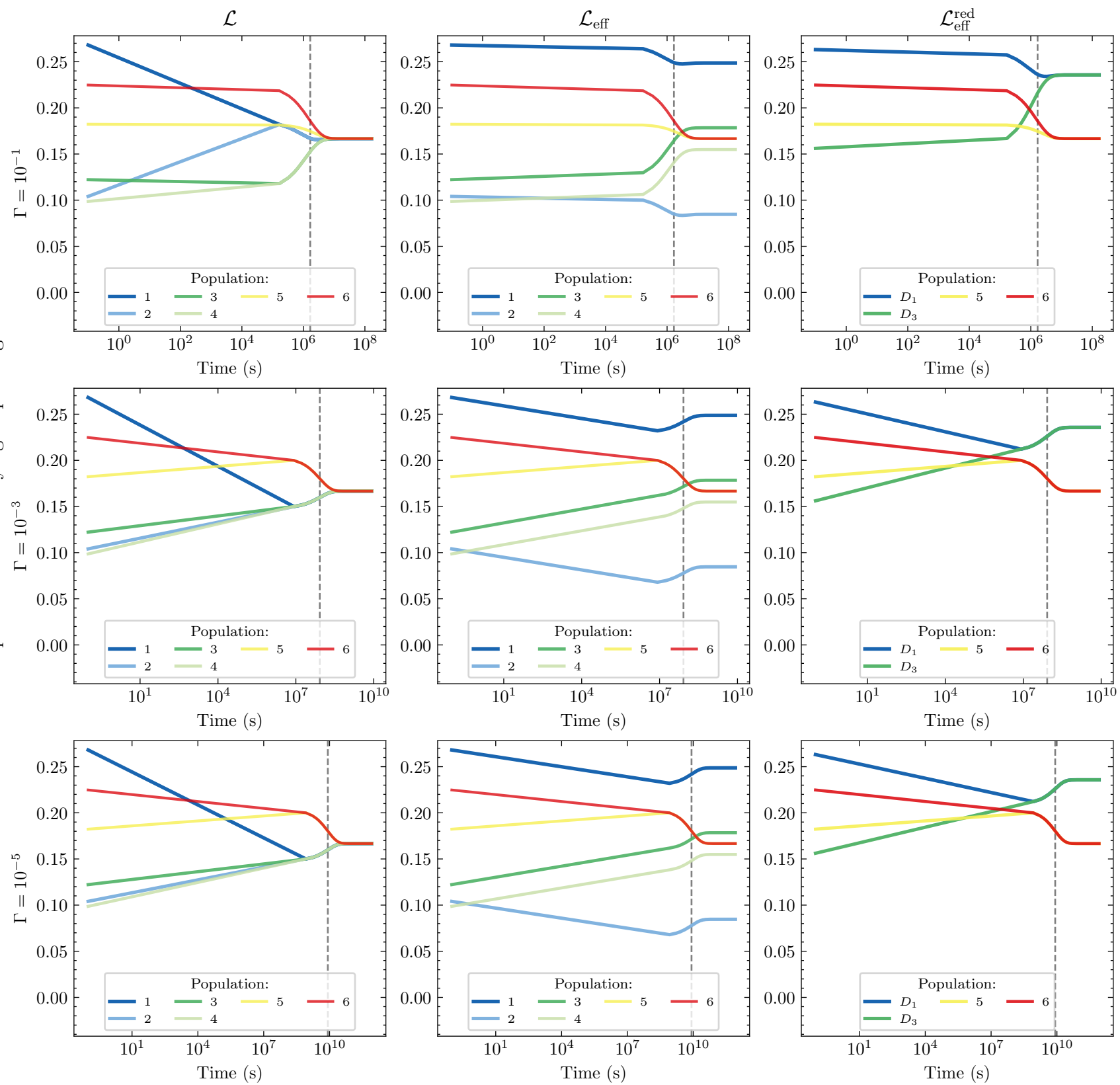
Time Evolution of Site Populations under \mathcal{L} , \mathcal{L}_{\text{eff}} , and \mathcal{L}_{\text{eff}}^{\text{red}} n_d=2 ; n_e=2 ; J = 10^{-1} ; \epsilon = 10^{-4}
